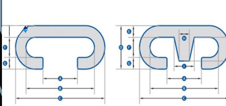
Selection dimensions of the various types of handrails (geometry specifications) in mm.
